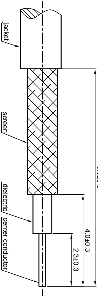
RECOMMENDED CABLE STRIPPING DIMENSIONS
